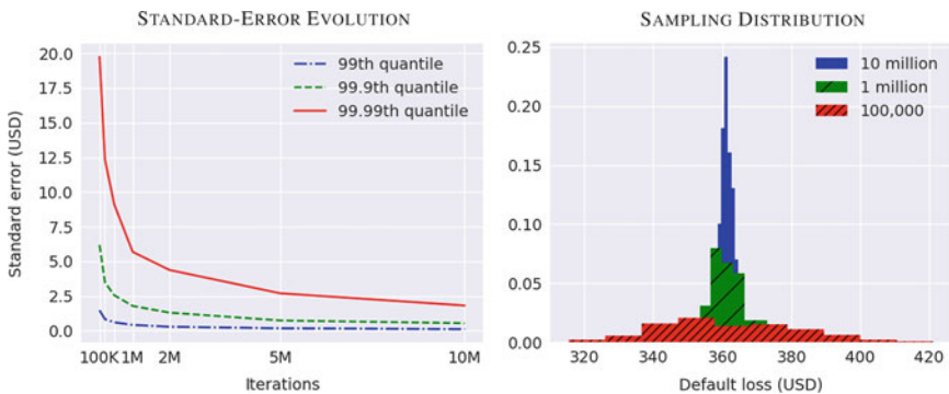
Fig. 8.7 Understanding convergence: The underlying figures provide two perspectives on the convergence properties of our Monte-Carlo estimator of the one-factor t -threshold model applied to our usual example. The left-hand graphic illustrates the reduction in standard error for a variety of levels of confidence as we increase the number of iterations, while the right-hand graphic highlights the sampling distributions for a fixed 99.99th quantile by various iteration settings.
