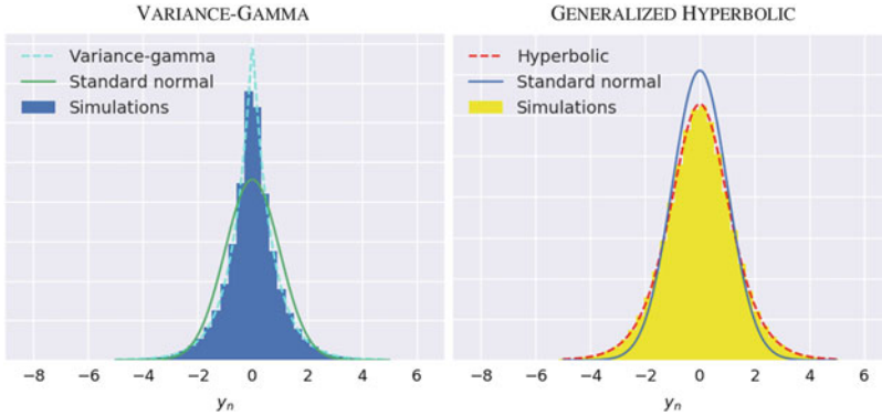
Fig. 4.10 Visualizing normal-variance-mixture distributions: This figure summarizes the theoretical and simulated variance-gamma and generalized-hyperbolic density functions. A standard normal density is also overlaid for comparison purposes.
