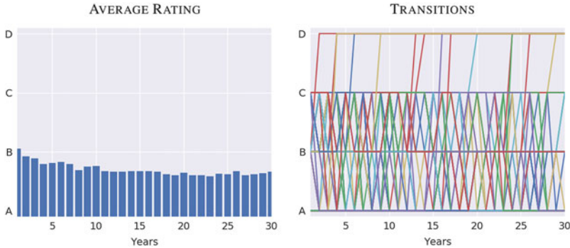
Fig. 9.5 Transition overview : The two graphics in this figure provide some insight into the characteristics of our simulated data. The left-hand graphic describes the average credit rating—it appears to be around the level of state B . The right-hand graphic, conversely, highlights the individual transitions for all of our 100 obligors. Observe that only a handful of default events occur.
