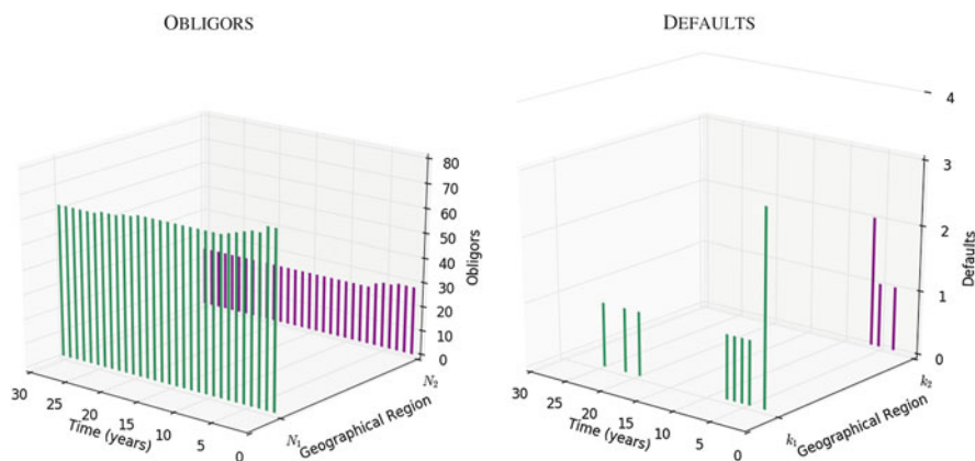
Fig. 10.8 Regional default data: These two figures illustrate the number of obligors, across our 30-year simulated dataset, and the incidence of default by counterparty and time period. In the vast majority of periods, no default event occurs.
