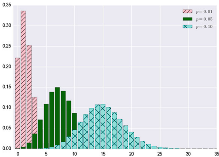
Fig. 2.3 Many instruments : This figure describe the distribution of default losses for a portfolio of 150 equally sized investments. Three possible common default-probability values are examined: 1, 5, and 10%.
