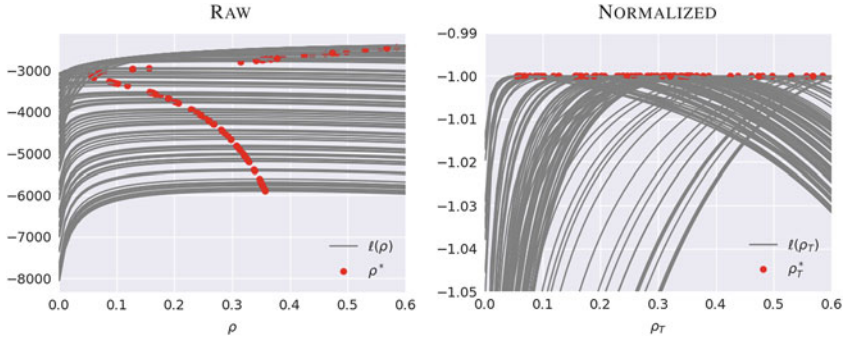
Fig. 10.12 Multiple log-likelihoods : Since we make K inference about the unobservable, latent, state variables, we generate K log-likelihood functions. It is still good practice to plot them and make a judgement on their granularity. The underlying graphics displays the consequences for K = 100 .
