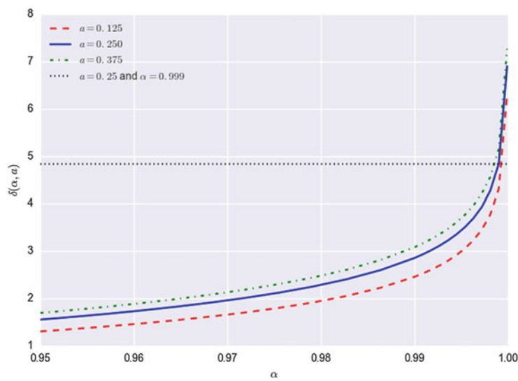
Fig. 6.11 Choosing \delta_\alpha(a) : This figure highlights the various values of \delta_\alpha(a) for \alpha levels in the range [0.95, 0.9999] for three possible choices of the a parameter: 0.125, 0.25, and 0.375. Currently, the recommended choice is to set a equal to 0.25.
