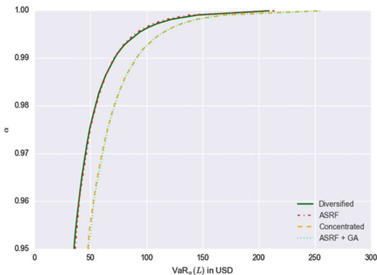
Fig. 6.10 Testing the granularity adjustment: This figure provides the tail probabilities for four different cases: the diversified ASRF, the concentrated ASRF, the one-factor Gaussian estimate of the diversified model, and the sum of the ASRF concentrated estimate plus the granularity adjustment. Both of our experiments are successful.
