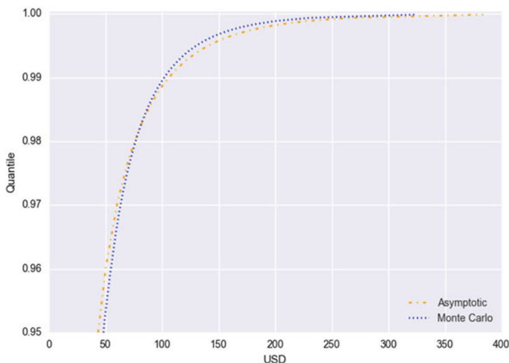
Fig. 4.5 The analytic fit: This figure compares the tail probabilities from the limit-loss analytic approximation and the full Monte-Carlo computation of the Gaussian threshold model. It confirms visually our conclusions from Table 4.2.
