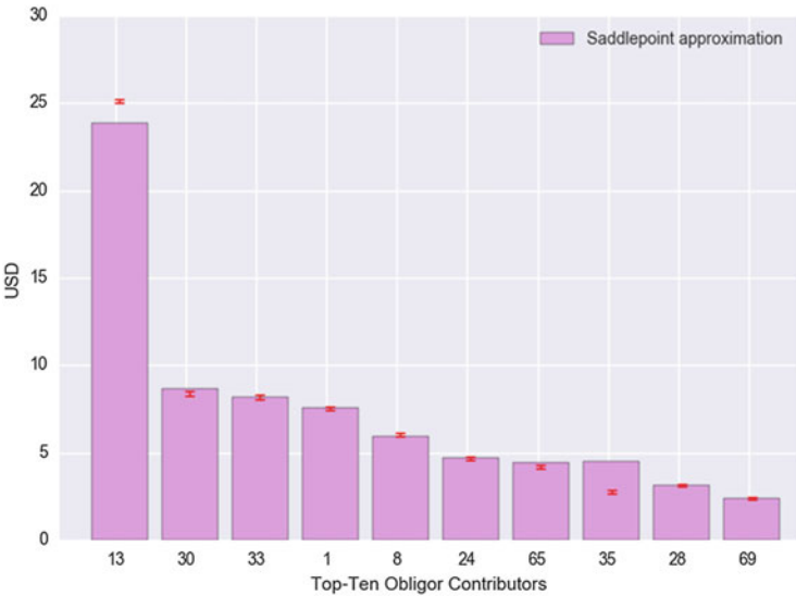
Fig. 7.11 Independent-default shortfall-contribution approximation: This figure outlines the saddlepoint expected-shortfall contribution approximations. They are compared with a Monte-Carlo estimate employing 500 million iterations. The red bars, as before, denote a 99% confidence interval around the Monte Carlo approximations.
