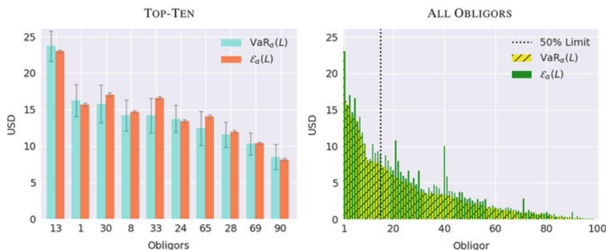
Fig. 7.1 Monte-Carlo obligor contributions : This figure illustrates the ten-largest and total obligor VaR and expected-shortfall contributions—ordered by their VaR contributions—for our running 100-obligor sample portfolio. All computations stem from a one-factor t -threshold model—a 95% confidence interval for the top-ten estimates is provided to underscore the noise in the estimates. About 50% of the total risk contribution arises from the 16 largest credit counterparts.
