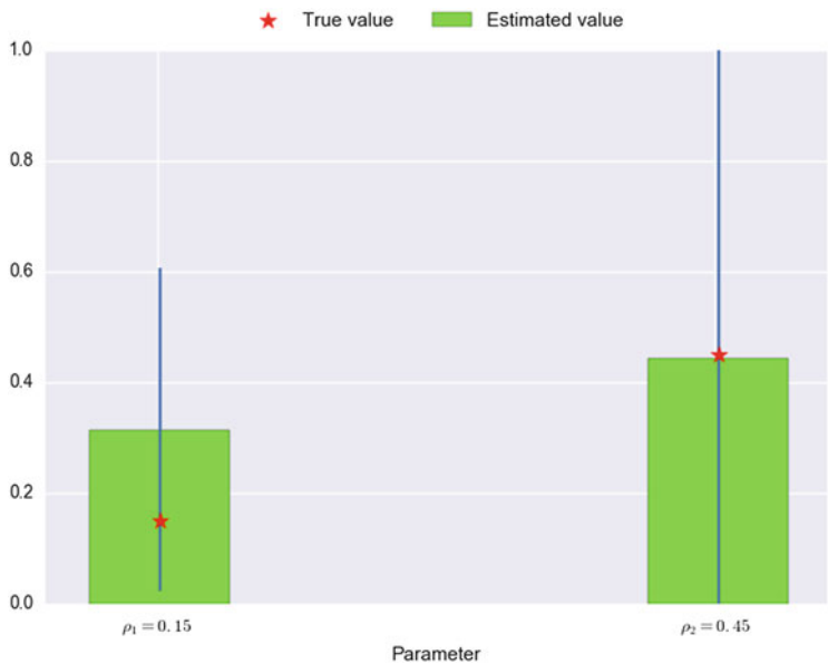
Fig. 10.11 Regional estimates: This figure illustrates graphically the main results of the regional simulation study found in Table 10.8.
