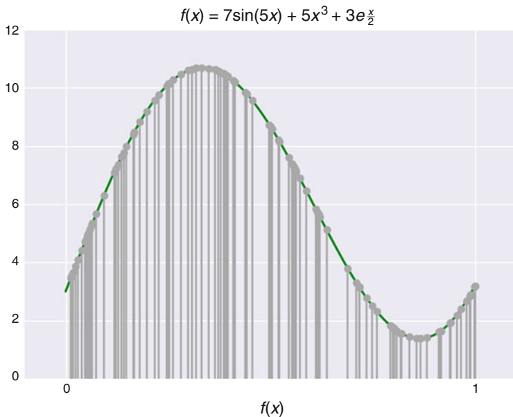
Fig. 8.4 A randomized grid: The underlying figure randomly draws 100 points for our silly function within the unit interval—our range of integration—from the standard uniform distribution. Although somewhat uneven, it does appear to cover much of the range.
