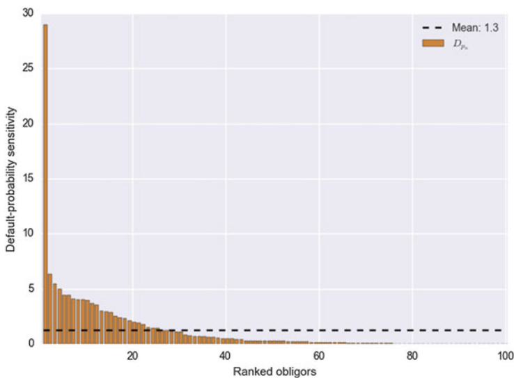
Fig. 9.2 Obligor differentiation : The underlying figure provides a visual perspective on the D_{p_n} estimates, from equation 9.4, for all 100 obligors in our sample portfolio. The average value is slightly greater than unity, although there are important differences across counterparties.
