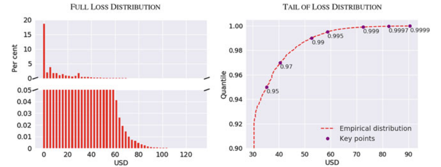
Fig. 2.5 The loss distribution: This figure outlines the full loss distribution for our simple 100-counterparty portfolio along with its tail from the 90th to the 99.99th quantile. The results from Table 2.4 are indicated.
