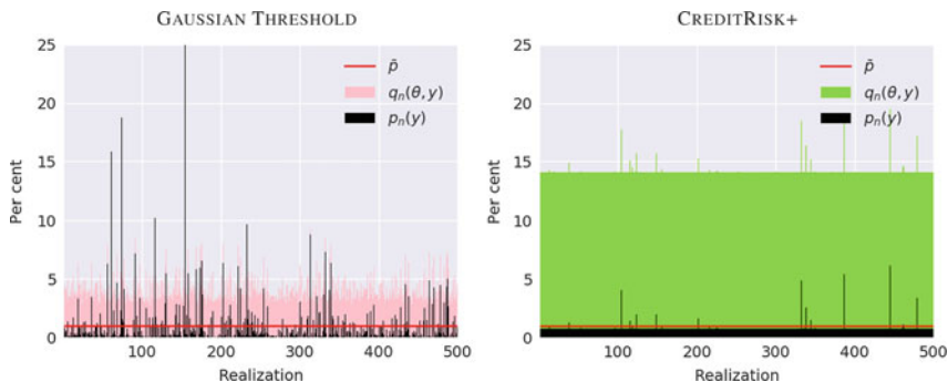
Fig. 8.9 Twisting probabilities : This figure illustrates the average twisted and non-twisted of conditional default probabilities for two competing models: the one-factor Gaussian threshold and one-factor CreditRisk+ approaches. In both cases, the \theta parameter was selected to force the mean of the default distribution to be equal to the 99.99th VaR quantile.
