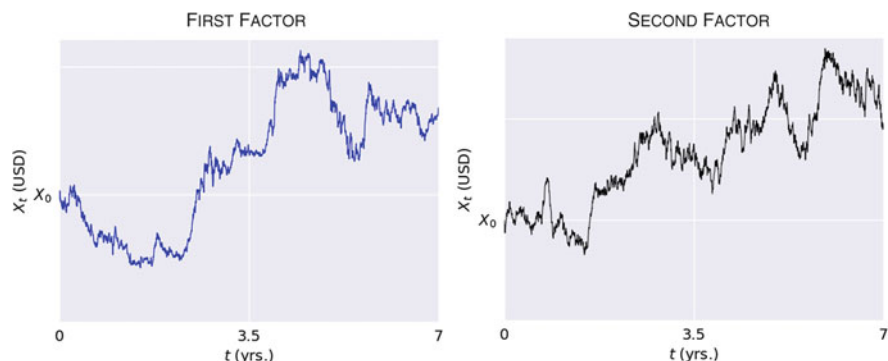
Fig. 1.4 Brownian motion in action : Examine the underlying risk factors. Which is a real, observed market-risk factor and which is a simulated path from a Brownian motion?
