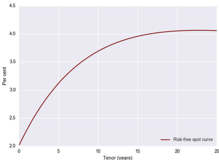
Fig. 9.15 An assumed risk-free spot curve: The underlying figure illustrates an assumed zero-coupon curve for our bootstrapping example. It is constructed using the Nelson and Siegel (1987) model with arbitrarily selected level, slope, and curvature parameters of 0.03, -0.01, and 0.05, respectively.
