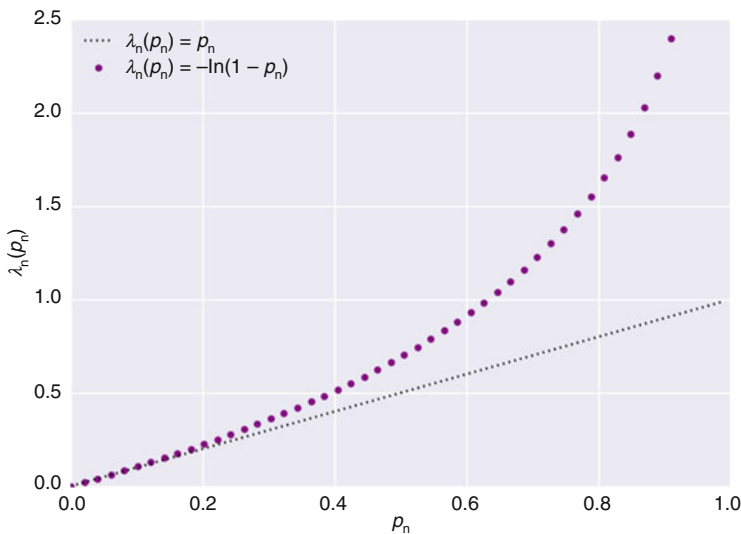
Fig. 2.7 Identifying \lambda_n : This figure outlines two different approaches toward identifying \lambda_n using the unconditional default probability, p_n . One is exact, whereas the other is an approximation. For small values of p_n , the differences are very small.
