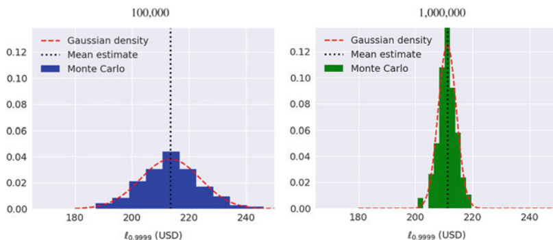
Fig. 8.6 The role of M : This figure illustrates the histogram of 200 separate estimations of the 99.99th quantile VaR of our sample portfolio using a one-factor Gaussian threshold model. The first estimate uses 100,000 iterations for each estimate, whereas the second employs 1 million. In each case, the distribution of Monte Carlo estimates is overlaid with a Gaussian distribution using the sample mean and sample error—the fit is quite reasonable.
