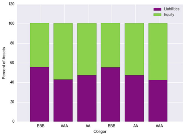
Fig. 5.7 Inferring the capital structure: These underlying figure provides, as a percentage of the total assets, the obligor-level liability and equity values. This clearly respects the constraint that A_t = L_t + E_t .
