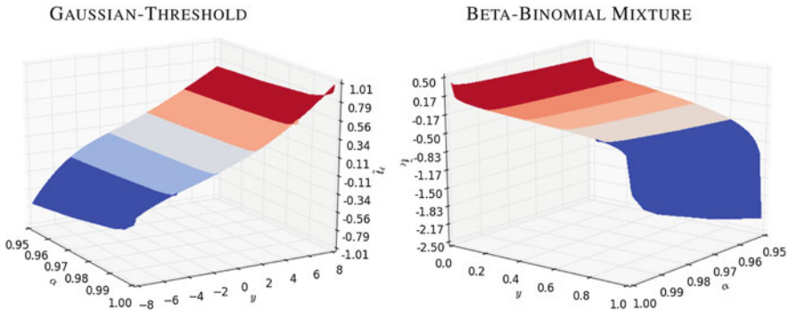
Fig. 7.12 Integrated saddlepoint density approximation: This figure illustrates, for two alternative models, the interplay between the level of confidence ( \alpha ), the value of the state variable ( y ), and the saddlepoint approximation ( \tilde{t}_\ell ). Unlike the independent-default case, the saddlepoint is negative for many values of y . As a consequence, we need to include some adjustments to our contour integrals to force them back through the origin.
