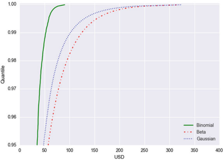
Fig. 4.3 Comparative tail probabilities: This figure provides a graphic description of the results found in Table 4.1. Observe how the beta-binomial and Gaussian threshold models converge in the tail.
