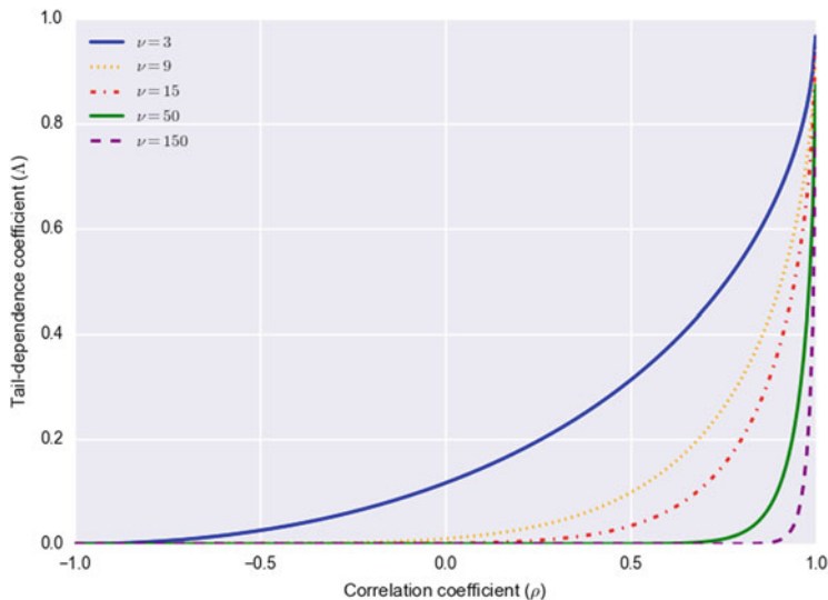
Fig. 4.6 Tail-dependence coefficients : This figure illustrates, for alternative choices of degrees-of-freedom parameters, the interaction between the correlation coefficient and the tail-dependence coefficient for the t -distribution summarized in equation 4.68. Observe that tail-dependence is an increasing function of the correlation coefficient, but a decreasing function of the degrees-of-freedom parameter.
