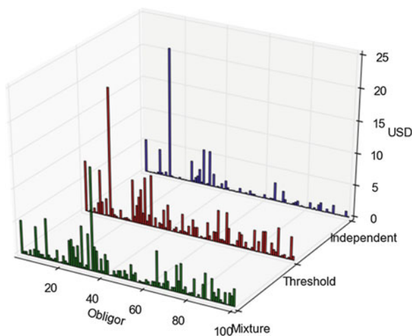
Fig. 1.11 Obligor VaR contributions: This figure outlines, for our three modelling choices, the contribution of each obligor to the overall 99.9th quantile VaR measure.
