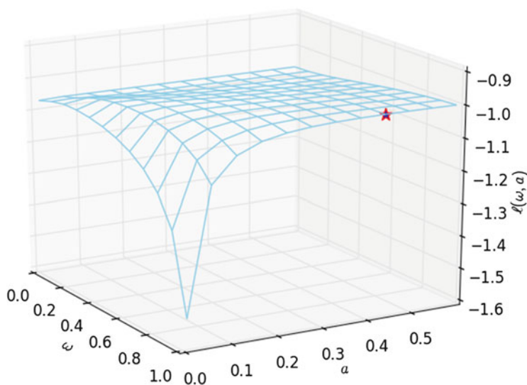
Fig. 10.6 The CreditRisk+ likelihood surface: The presence of two CreditRisk+ model parameters directly implies a two-dimensional likelihood function. This allows us to visually determine the regularity of the log-likelihood.
