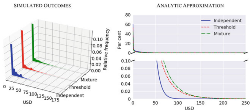
Fig. 1.9 Default-loss distributions: These graphics highlight—for our sample portfolio—the default-loss distribution estimated with three alternative credit-risk models.
