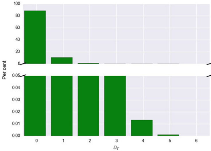
Fig. 5.9 Direct Merton-model default-loss distribution: For our six-counterparty example with default correlation, this graphic details the distribution of the number of losses. Almost all of the probability mass occurs at 0-1 defaults; we had to zoom in the axis to under 5 basis points to permit visibility of the distribution's tail.
