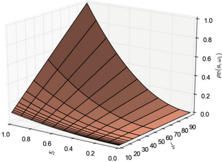
Fig. 3.9 A default-correlation surface: The underlying figure outlines the relationship between the default correlation described in equation 3.86 and its parameters. The highest levels of default correlation are achieved when \omega_1 and \frac{1}{a} are simultaneously large. In all cases, we have assumed that p_n = p_m = 0.01 . Understanding this fact helps us sensibly calibrate this model.
