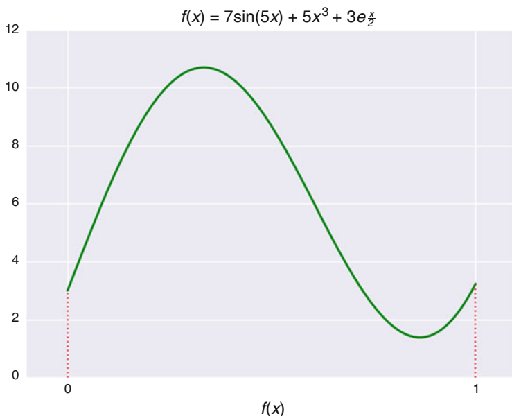
Fig. 8.1 A silly function : The underlying figure summarizes the behaviour of the function summarized in equation 8.4 over the unit interval.
