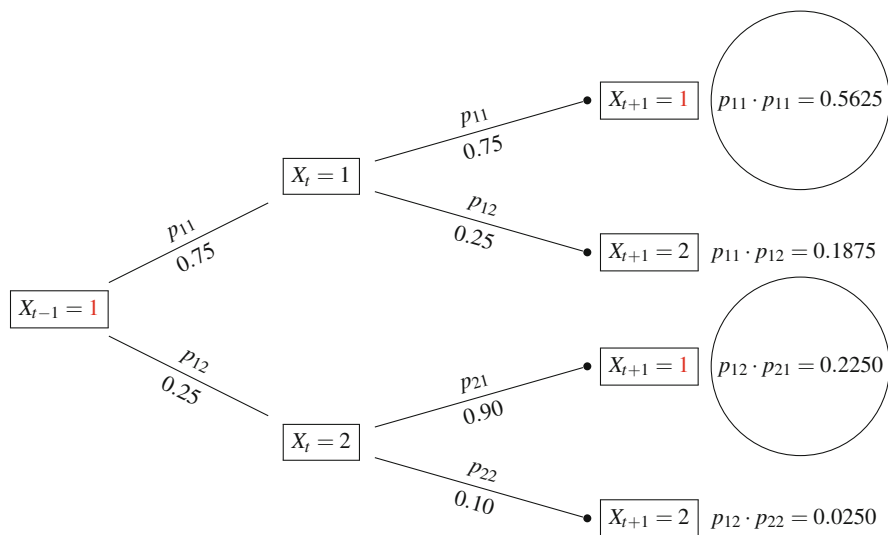
Fig. 9.3 Calculating forward Markov-Chain probabilities: The underlying schematic diagram constructs a two-step tree diagram outlining the various outcomes of a two-state Markov chain. This allows us, with some book-keeping, to determine \mathbb{P}(X_{t+1} = 1 | X_{t-1} = 1) .
