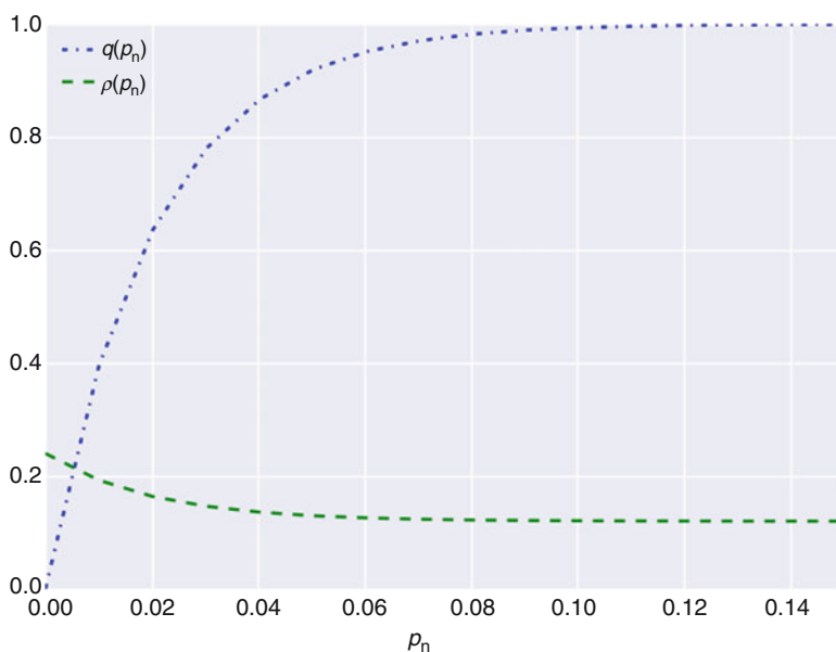
Fig. 6.1 Basel asset correlation : This figure outlines the weighting function, q_n , from equation 6.12 and the associated asset correlation estimate—from equation 6.11—for different levels of unconditional default probability. For values of p_n greater than about 0.12, the \rho_n parameter takes the value of \rho^- or 0.12.
