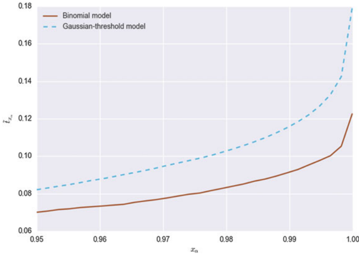
Fig. 7.5 Saddlepoint positivity : This figure computes the saddlepoint values for a range of confidence levels \alpha \in [0.9500, 0.9999] . We will discuss precisely how this is implemented in the following sections, but we first wish to establish that it generally takes a positive value.
