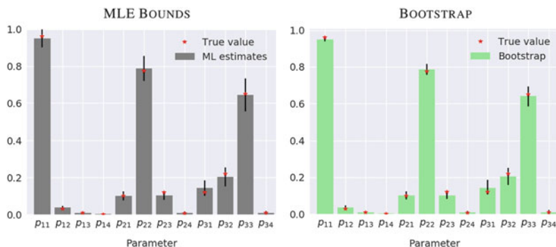
Fig. 9.12 Comparing approaches : The two underlying graphics display the estimates of each transition probability along with true values and a 95% confidence interval for the MLE and bootstrap approaches, respectively. The results are, visually at least, in broad agreement.
