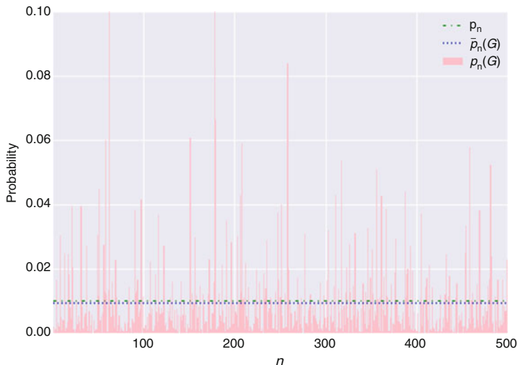
Fig. 4.2 p_n(G) dynamics: This figure assumes a value of p_n = 0.01 and \rho = 0.2 . It then simulates 500 random draws of G \sim \mathcal{N}(0, 1) and computes the associated conditional default probabilities. We see, quite clearly, that the default probability has been randomized.
