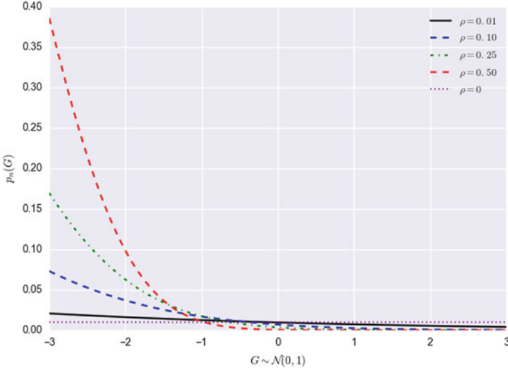
Fig. 4.1 Conditional default probability : This figure uses the conditional default probability, as described in equation 4.18, to demonstrate the impact of the value of G . As G takes on large negative values, it leads to monotonically greater conditional default probabilities. The effect increases for increasing values of \rho .
