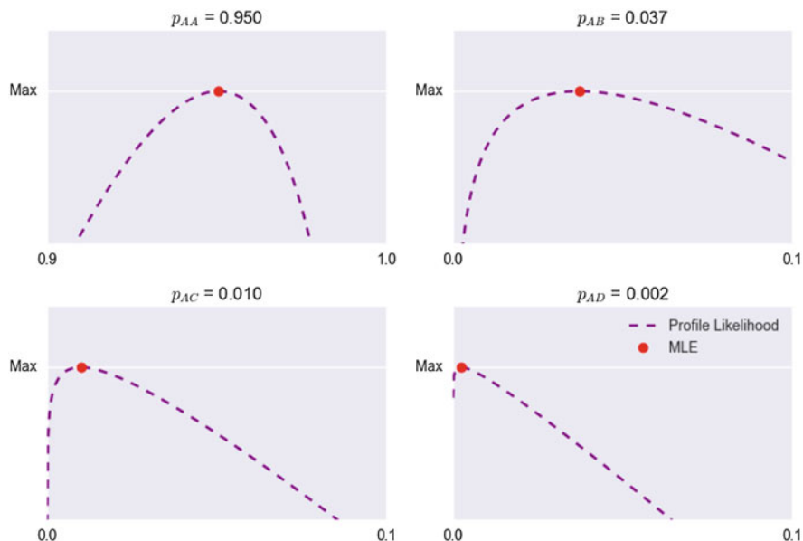
Fig. 9.9 Likelihood curvature : As highlighted in Pawitan (2001), the larger the curvature around the maximum of the likelihood function, the higher the implied level of parameter certainty. The figure magnifies the results from Fig. 9.8 to help us visualize the degree of MLE-curvature for each of the four estimates in the first row of \hat{P} .
