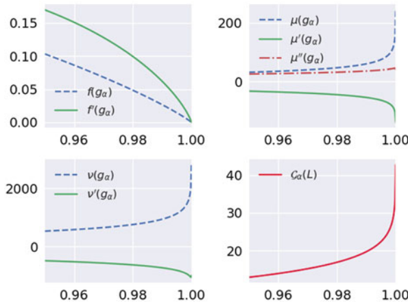
Fig. 6.8 Gaussian granularity adjustment functions : The underlying figure highlights, over the range \alpha \in (0.95, 1.00) , the form of the various functions derived in the preceding pages. There are significant differences in scales and forms of these functions and their derivatives. All values are evaluated at the appropriate quantile value for the underlying systematic variables: g_\alpha = q_{1-\alpha}(g) .
