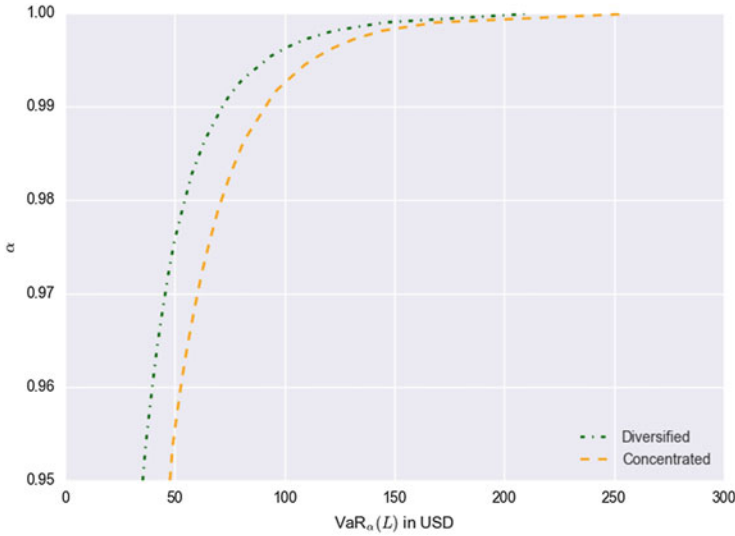
Fig. 6.9 Concentrated vs. diversified tail probabilities : This figure highlights the tail probabilities over the range [0.95, 0.9999] for the diversified and concentrated portfolios summarized in Table 6.4. All estimates are computed using the one-factor Gaussian threshold model with a common \rho parameter equal to 0.19.
