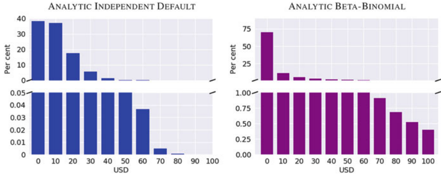
Fig. 3.1 The role of default dependence: This figure compares the loss distributions from the independent-default and beta-binomial mixture models. Both models are nested. The beta-binomial has, however, randomized the default probability and induced a default dependence on the order of 0.05. The differences are striking.
