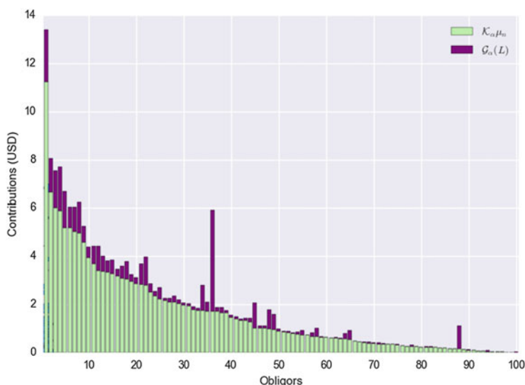
Fig. 6.13 Revisiting economic-capital contributions: This figure returns to the base Basel IRB contributions provided in Fig. 6.6 and, using the previously described granularity adjustment approach, adds the concentration-risk contributions.
