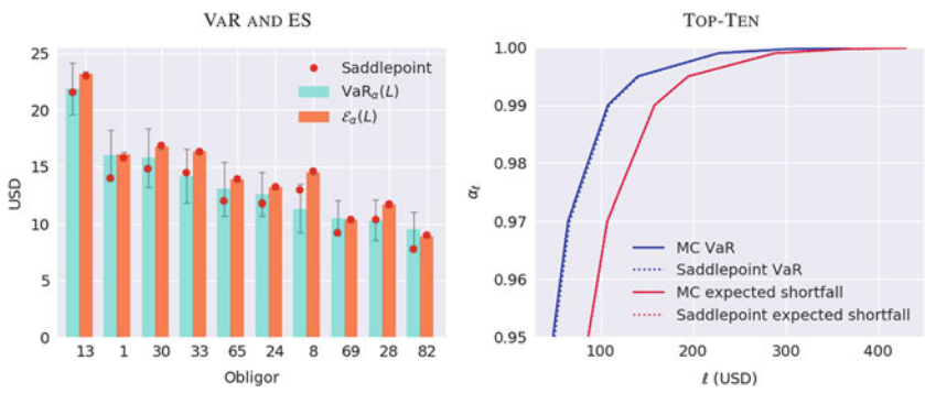
Fig. 7.16 Back to the beginning: The t -threshold model: This figure returns to the Monte-Carlo estimates of the ten largest one-factor t -threshold VaR and expected-shortfall contributions. For comparison purposes, it shows the associated saddlepoint approximations computed using two-dimensional numerical integration. It also demonstrates the accuracy of the saddlepoint tail-probability and shortfall-integral estimates.
