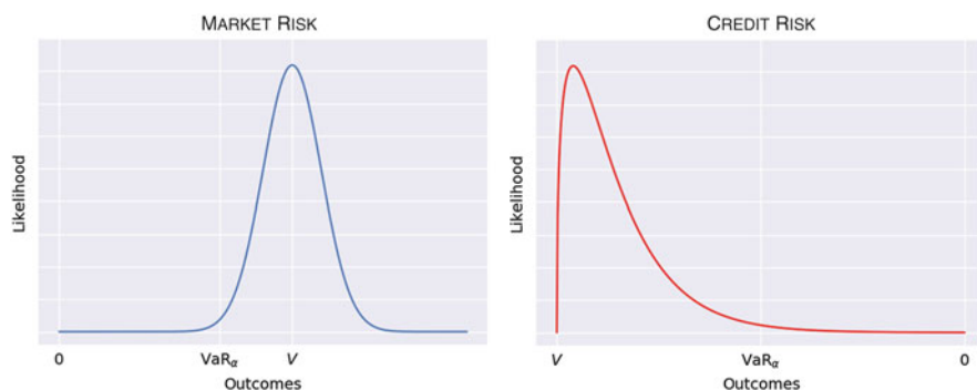
Fig. 1.6 A stylized comparison: Due to their fundamental differences, profit-and-loss outcomes and their associated likelihoods are combined in alternative ways in the market- and credit-risk settings.
