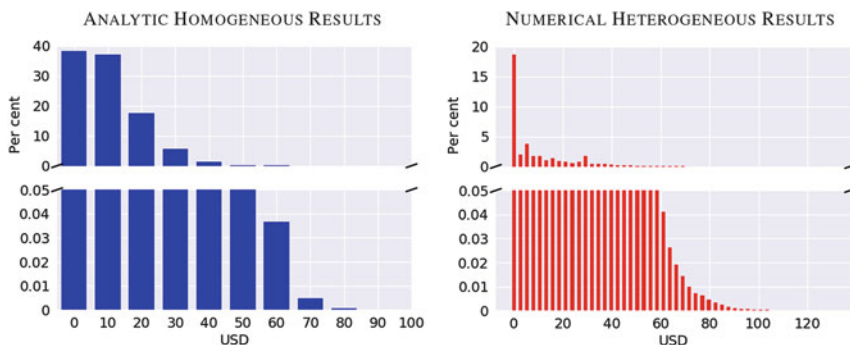
Fig. 2.6 Impact of homogeneity assumptions: This figure outlines the full loss distribution for the analytic solution, with its embedded homogeneity assumptions for default probabilities, against the heterogeneous numerical results found in Fig. 2.5.
