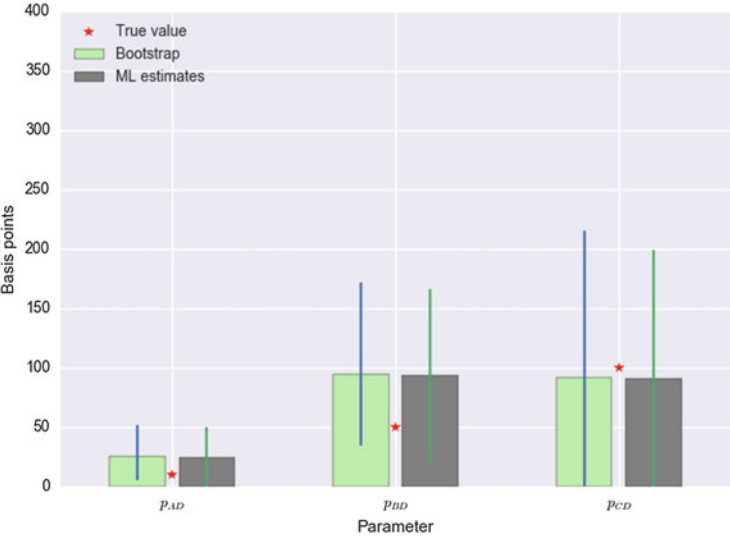
Fig. 9.13 Default-probability confidence bounds: This figure takes the default probability results from Fig. 9.12 and magnifies them providing a closer look. We may conclude that, in this instance at least, the bootstrap provides a more accurate and conservative assessment of parameter uncertainty.
