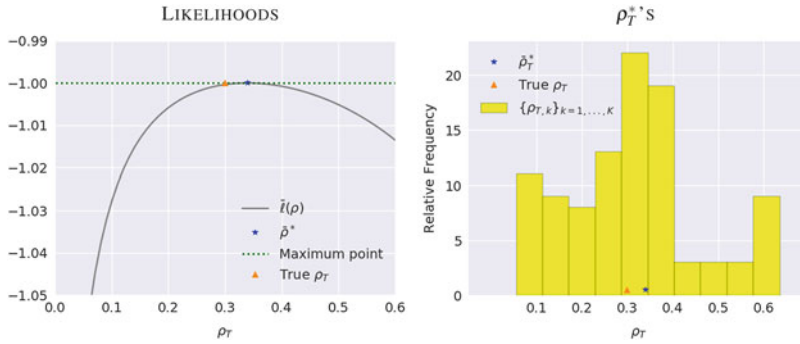
Fig. 10.13 Averaging log-likelihoods : Fig. 10.12 is interesting and informative, but it is also useful to consider the average result. The average, after all, forms our final estimate. The underlying graphics, therefore, illustrate the average log-likelihood function and the distribution of \rho_T estimates.
