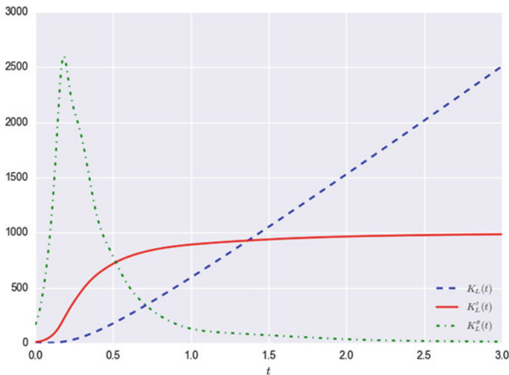
Fig. 7.6 Cumulant generating function and derivatives: This figure highlights, for a portfolio of 100 randomly generated heterogeneous exposures and default probabilities, the cumulant generating function and its first two derivatives. Note that K'_L(t) is a monotonically increasing function of t .
