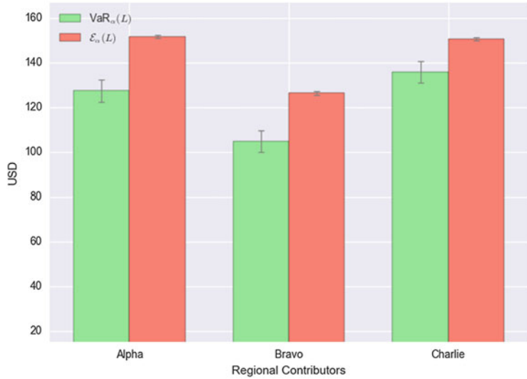
Fig. 7.2 Regional contributions: This figure illustrates the regional VaR and expected-shortfall contributions for our running 100-obligor sample portfolio; the computations stem from a one-factor Gaussian threshold model.
