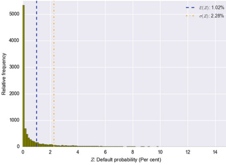
Fig. 3.2 Simulating beta random variables: This figure illustrates a histogram of 10,000 beta-distributed random variates with parameters \alpha = 0.2 and \beta = 18.9 . The outcomes were generated from the relationship found in equation 3.30.
