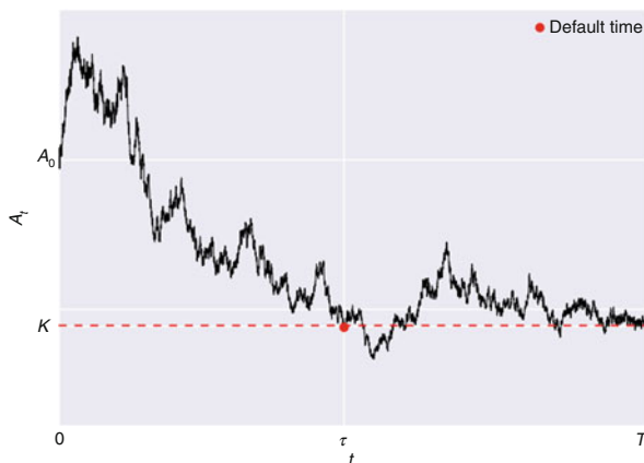
Fig. 1.5 Brownian motion in credit risk: Geometric Brownian motion can, and often does, arise in the credit-risk setting. It plays, however, a rather different role.
