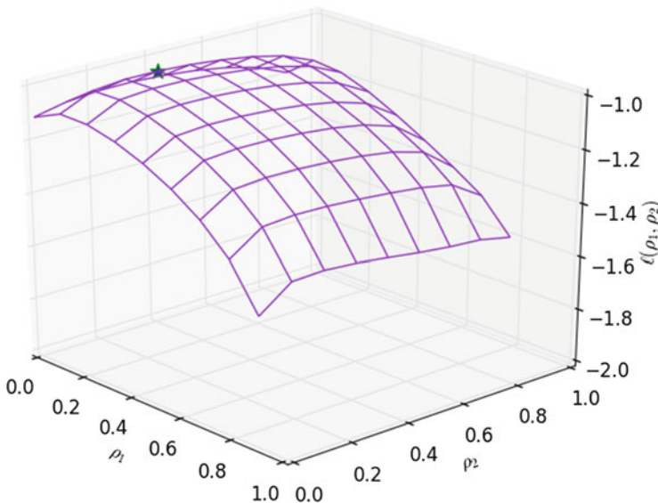
Fig. 10.9 The regional likelihood surface: Given that we have a two-dimensional likelihood function, we may plot the overall likelihood surface. This allows us to visually determine the regularity of the log-likelihood.
