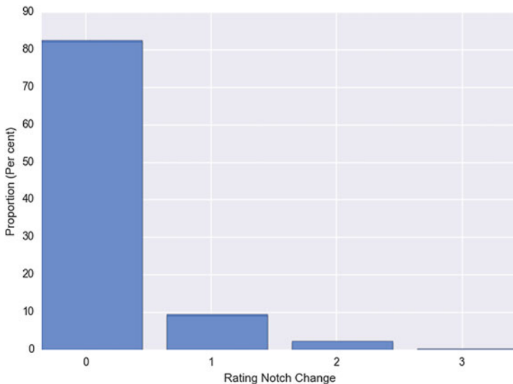
Fig. 9.6 Type of transitions : This figure displays a histogram of the transitions from our simulated data. Almost 80% of the time, an obligor remains in its current state. About 10% of the cases involve a one-state transition. Very few two-state transitions and a vanishingly small number of three-state transitions occur.
