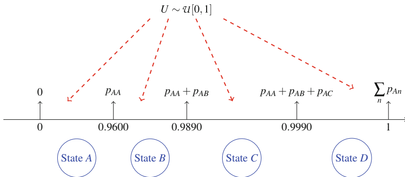
Fig. 9.4 Simulating a Markov chain: The simulation of a Markov chain is conceptually similar to the generation of a Bernoulli trial, albeit with more possible outcomes. First, one draws a standard uniform random variate, U \sim \mathcal{U}[0, 1] . Then, we use the row of the transition matrix corresponding to the current state—in this case, state A—to partition the unit interval. The outcome of U , as described in the underlying figure, determine the new state.
