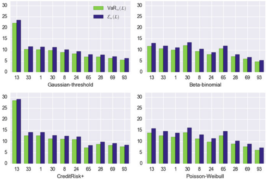
Fig. 7.14 Saddlepoint risk-measure contributions : This figure graphically shows the top-ten 99.99th quantile VaR and expected-shortfall contributions for each of our four models. The various approaches exhibit rather different implications for the individual contributions of specific obligors. All values are in USD.
