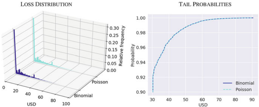
Fig. 2.8 Indistinguishable : This figure compares both the loss distribution and its tail probabilities for identically calibrated binomial and Poisson independent-default models. The results, while not exact, are visually indistinguishable.
