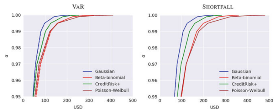
Fig. 7.13 Multiple-model visual risk-metric comparison: This figure graphically depicts the application of the saddlepoint approximation—for both VaR and expected-shortfall estimates—across four alternative models. The saddlepoint estimates are quite accurate and improve as we move further out into the tail.
