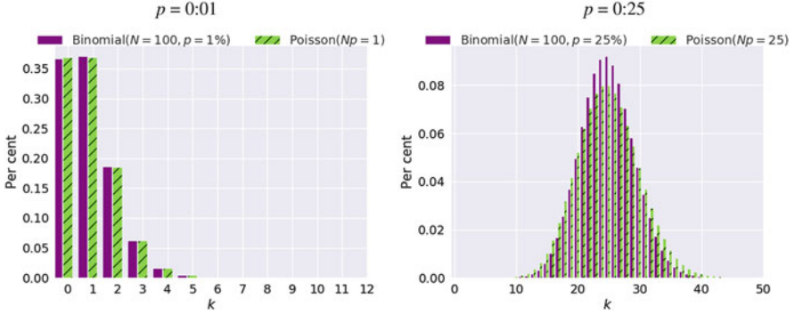
Fig. 2.9 The law of rare events : This figure compares, for different choices of p and N , the binomial and Poisson distributions. For sufficiently small \lambda = pN , the results are almost indistinguishable; this is referred to as the law of rare events.
