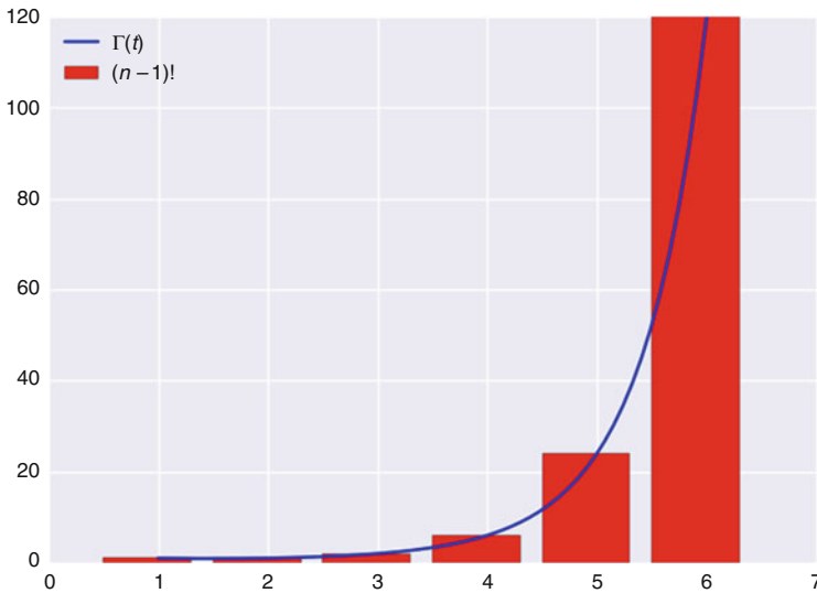
Fig. 3.6 The gamma function: This figure provides a very rough visual justification for the relationship between the gamma function and the factorial operator. For a fascinating description of the origins and history of this special function, see Davis (1959).
