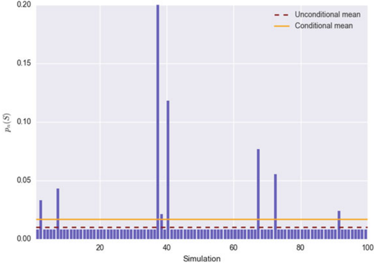
Fig. 3.8 CreditRisk+ conditional default probabilities : This graphic summarizes 100 random simulations of the CreditRisk+ conditional default probability with \omega_1 = 0.2 , a = 0.01 , and p_n = 0.01 . 80% of the weight is on the idiosyncratic factor, which implies that p_n(S) is often around 80 basis points, but occasionally a large outcome of S pulls it up above this level.
