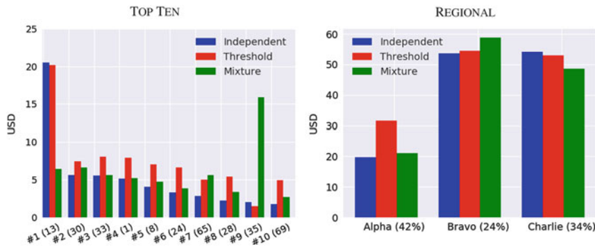
Fig. 1.12 VaR contribution perspectives: These two graphics demonstrate two alternative perspectives that might be applied to the obligor-level 99.9th quantile contributions: the top-ten contributors and the regional breakdown.
