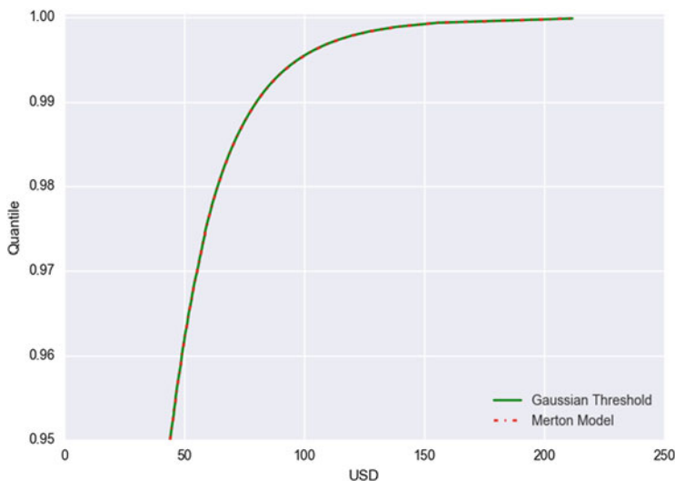
Fig. 5.6 Comparing tail probabilities: If one uses default probabilities to infer the default barrier, as done in Fig. 5.5, the Merton (1974) approach reduces to a one-factor threshold model. The figure below indicates that, visually, there is no difference in the tail probabilities.
