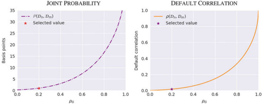
Fig. 10.2 Choosing \rho_G : This figure highlights the joint-default probability and default correlation for a variety of choices of the parameter \rho_G with an average starting default probability of approximately 50 basis points.
