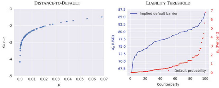
Fig. 5.5 Inferred quantities : Given the (assumed) asset-return information in Table 5.2, we can use p_n to infer K_n and the distance-to-default. The underlying graphics examine the relationship, on an obligor level, between these two inferred quantities and the default probabilities.
