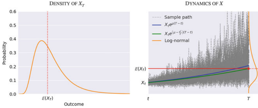
Fig. 5.4 SDE behaviour : Fig. 5.2 demonstrates the behaviour of the ordinary-differential element of geometric Brownian motion. These two figures describe the density and dynamics when the diffusion component is included; this dramatically changes the story.
