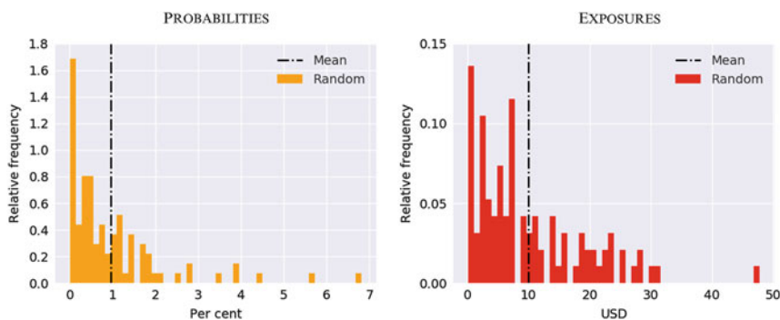
Fig. 1.7 A sample portfolio: The underlying graphics illustrate the individual exposures and unconditional default probabilities associated with our 100 obligor asset portfolio.
