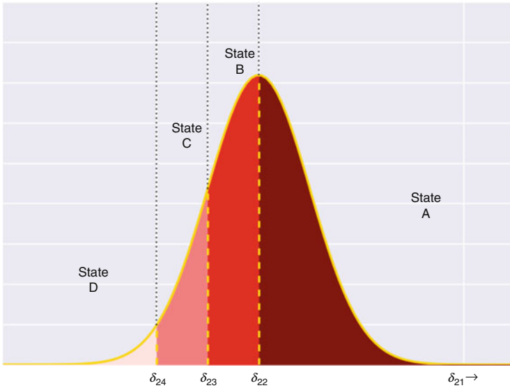
Fig. 10.1 Creating transition data: This figure visually illustrates the creation of the transition dataset. The transitions are delineated by a partition of the domain of the standard normal variable following the appropriate row in the transition matrix. The underlying schematic relates to a fictitious row of an arbitrary four-dimensional Markov chain with transition matrix, P .
