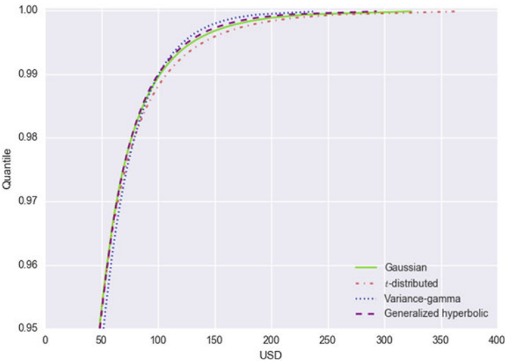
Fig. 4.11 Multiple threshold tail probabilities: This figure summarizes the tail probabilities for the four one-factor threshold models considered in this chapter: the Gaussian, t , variance-gamma, and generalized-hyperbolic approaches. Visually, the models generate quite similar results.
