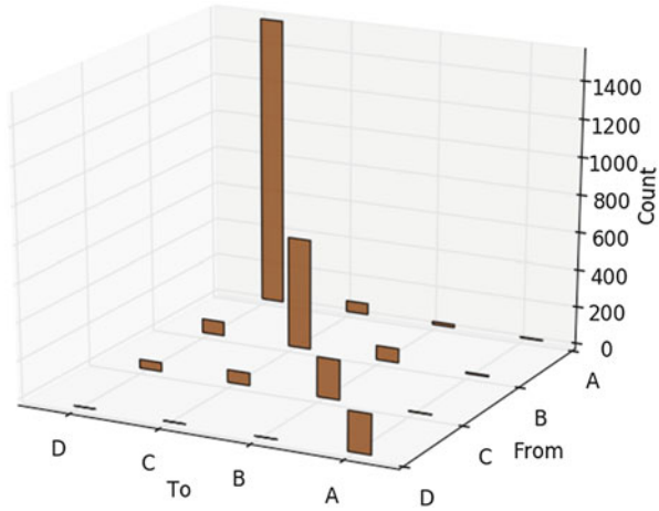
Fig. 9.7 Simulated transition counts : Using Algorithm 9.2, we count the number of possible transitions from our simulated credit-quality data. The underlying three-dimensional figure highlights the distribution of these counts.
