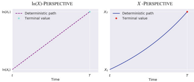
Fig. 5.3 ODE behaviour : These two figures graphically describe the behaviour—both with and without natural logarithms—of the embedded ordinary differential equation found in geometric Brownian motion.
