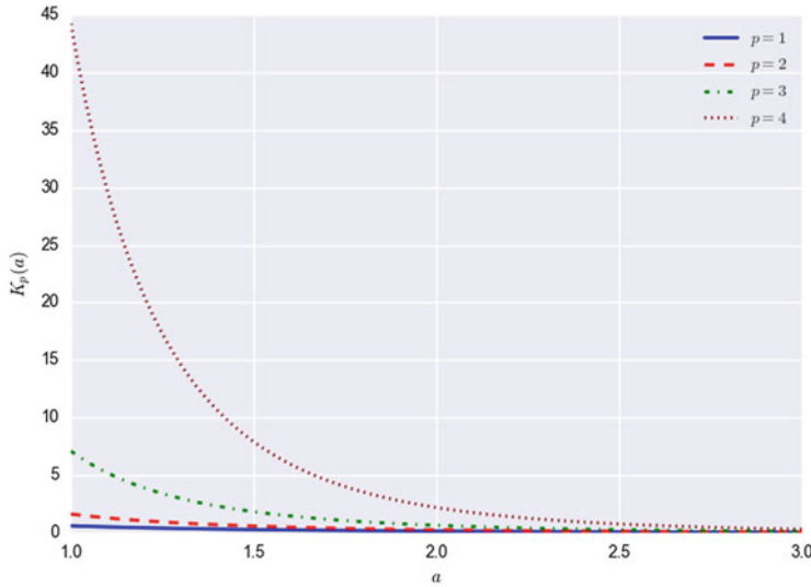
Fig. 4.9 The modified Bessel function of the second kind: This figure illustrates, for different choices of parameters a and p , the form of the modified Bessel function of the second kind.
