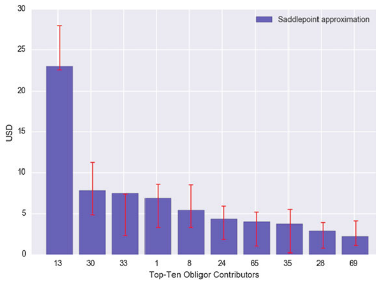
Fig. 7.9 Independent-default VaR-contribution approximation : This figure outlines—for our usual portfolio of randomly generated heterogeneous exposures and default probabilities—the saddlepoint VaR-contribution approximations. They are compared with a Monte-Carlo estimate employing 100 million iterations. Recall that the total portfolio values $1,000 and the red bars denote a 99% confidence interval around the Monte Carlo approximations.
