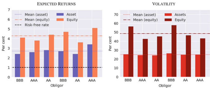
Fig. 5.8 Equity and asset moments: These two figures graphically compare, for each of the six obligors in Table 5.6, the asset and equity expected returns and volatility.
