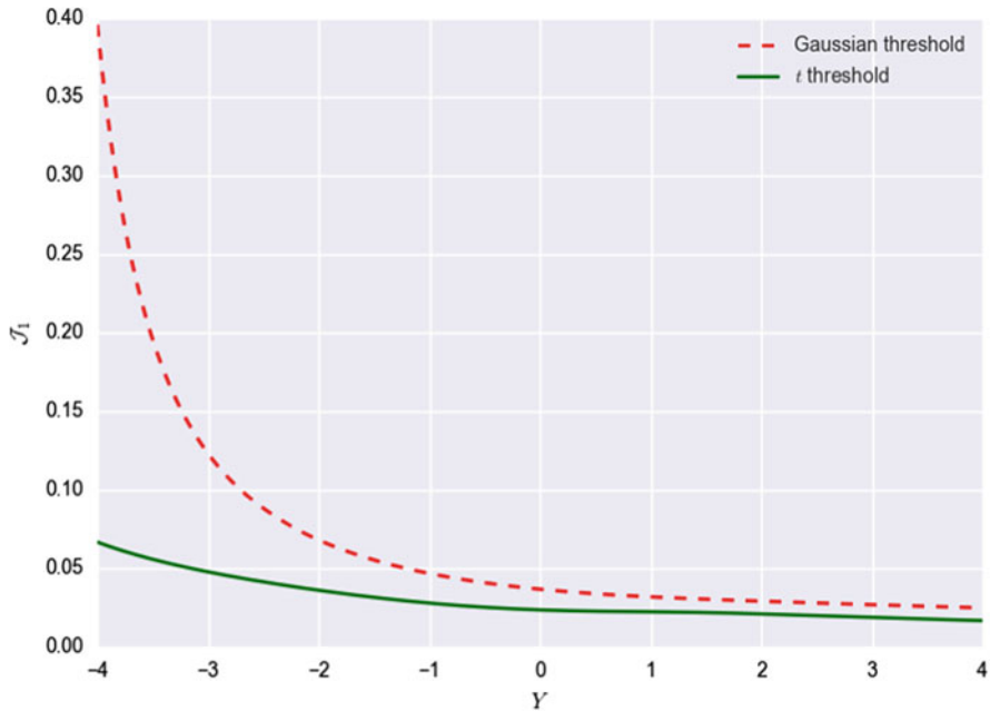
Fig. 8.11 \mathcal{J}_1 behaviour: This figure illustrates the evolution of \mathcal{J}_1 function for the 99.99th quantile of the Gaussian and t -threshold models across a broad range of state variable values. In both cases, we observe that it remains significantly below unity supporting the upper bound employed in equation 8.65.
