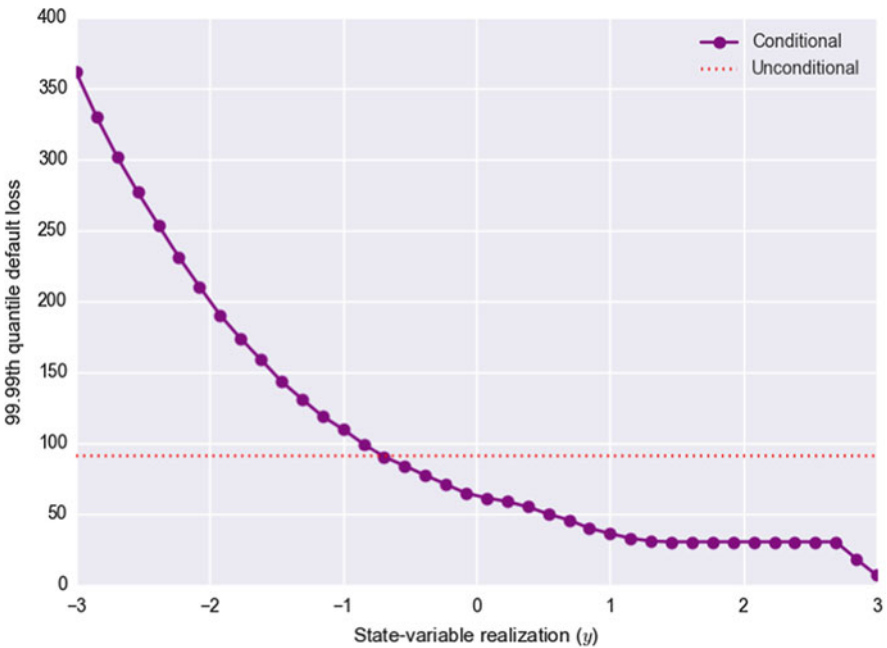
Fig. 8.10 Conditional VaR : This figure illustrates the evolution of the 99.99th quantile of the loss distribution conditioning each time on a different, but fixed, level of the state variable, Y = y . The results, presented for the one-factor Gaussian model, are compared to the unconditional VaR, which is basically the average across all state-variable outcomes. Similar patterns are evident in all previously examined threshold and mixture models.
