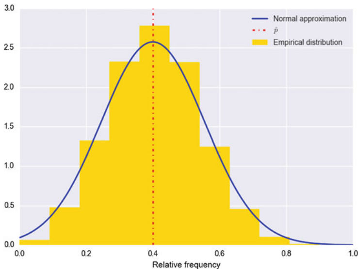
Fig. 9.11 Binomial bootstrap distribution : This figure summarizes the bootstrap distribution of \hat{p}^* associated with 10,000 simulated samples of 10 observations. For perspective, the maximum-likelihood estimator and normal approximation are also illustrated. There is strong agreement among the results.
