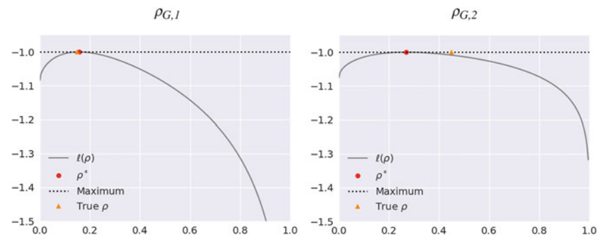
Fig. 10.10 Regional profile likelihoods: As a complement to the full two-dimensional likelihood, illustrated in Fig. 10.9, this figure highlights the profile likelihoods for each parameter. Profile likelihoods are computed by tracing out the likelihood function for all values of one parameter, while holding other parameters fixed at their maximum-likelihood estimator.
