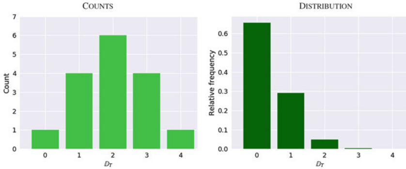
Fig. 2.1 Four-instrument outcomes : This figure illustrates the individual default counts along with the default-loss distribution for the four-instrument example detailed in Table 2.3.
