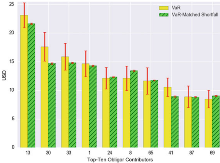
Fig. 7.3 VaR-matched comparison : This figure compares—for \alpha^* \approx 0.9997 —the ten largest VaR and VaR-matched expected-shortfall contributions for the t -threshold one-factor also displayed in Fig. 7.1.
