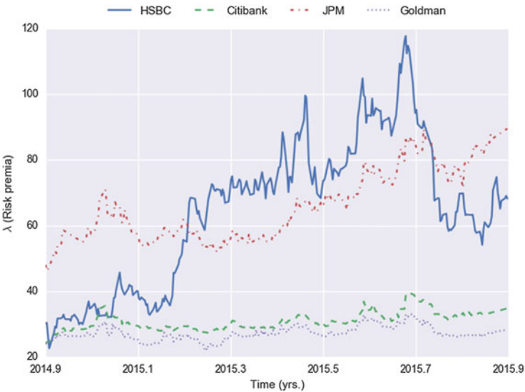
Fig. 9.18 Approximate risk-premium evolution: This figure highlights, for illustrative purposes, the approximate evolution of the risk premium over our sample period. The risk-neutral default probabilities change with each observation, while the values under the physical measure are held fixed.
