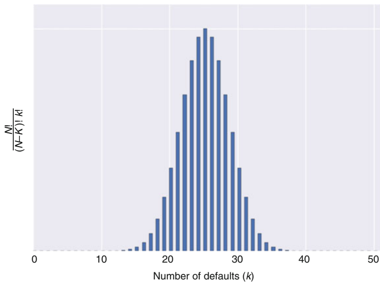
Fig. 2.2 Pascal's triangle : This figure illustrates the sequence of binomial-coefficient values associated with \binom{50}{k} for k = 0, \dots, 50 ; this is the 50th row of what is often referred to as Pascal's triangle. Its basic shape should appear relatively familiar.
