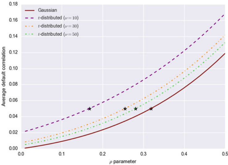
Fig. 4.7 Calibrating outcomes : This figure illustrates—for the Gaussian and selection of t -distributed models each with a differing degrees-of-freedom parameter, \nu —the relationship between the average default correlation and the single model parameter, \rho . As \nu \rightarrow \infty , the t -distributed calibration converges to the Gaussian. The black stars denote the optimal \rho value associated with our target of \rho_D = 0.05 .
