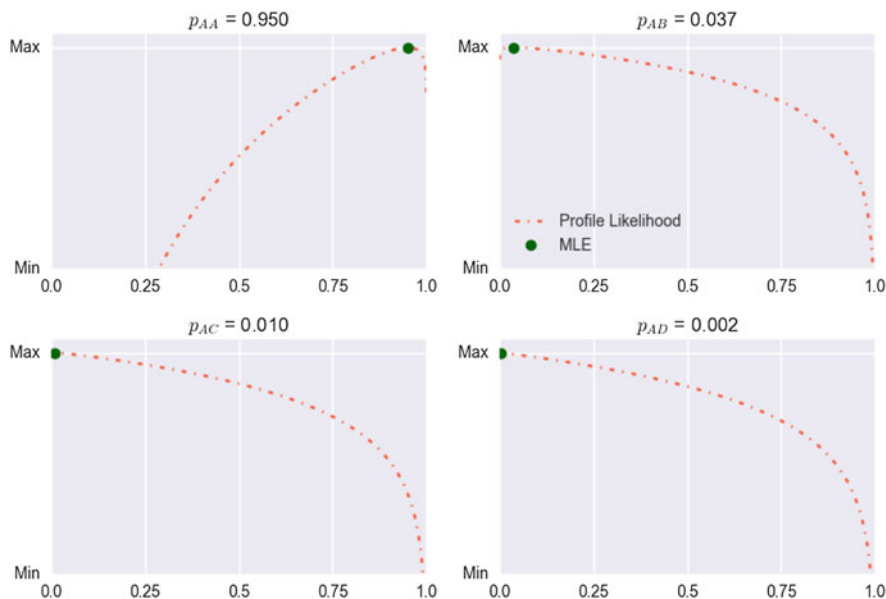
Fig. 9.8 The profile likelihood : Graphing the likelihood function provides important insight into the certainty of one's parameter estimates. In a multivariate setting, this is challenging. The profile likelihood addresses this issue by examining one parameter at a time—this figure examines the four parameters of the first row of P .
