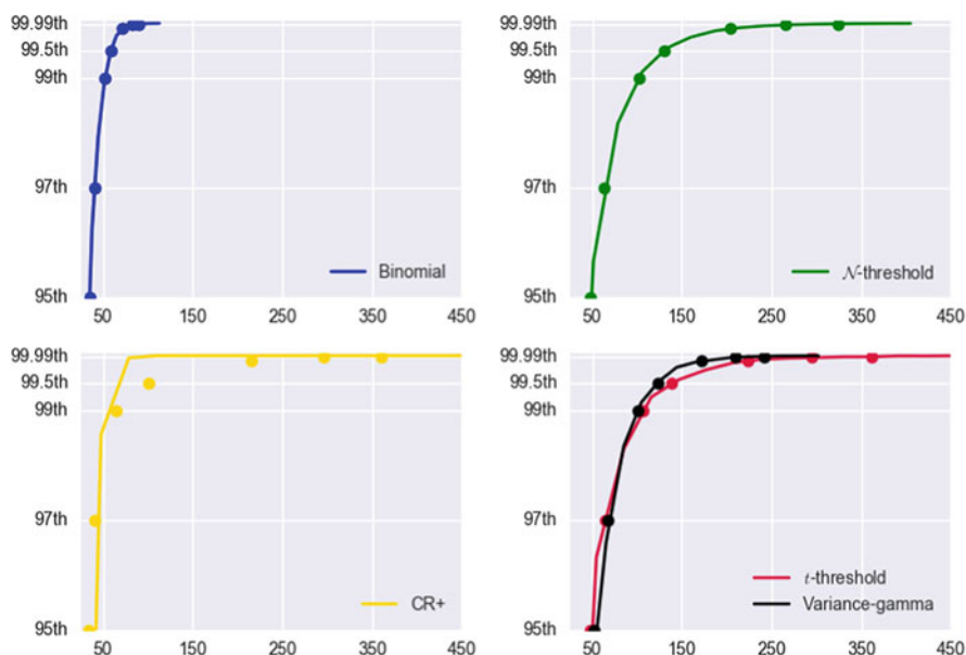
Fig. 8.14 Raw vs. IS VaR comparison: This figure compares the raw and importance-sampling VaR estimates and associated tail probabilities across five alternative models using our usual 100-obligor example. The IS values are computed with 50 repetitions of 3,000 iterations, whereas the raw simulation values involve 250 repetitions of 10 million iterations.
