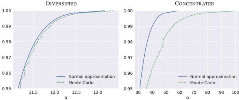
Fig. 7.4 Accuracy of normal VaR approximation: This figure outlines the accuracy of the normal VaR approximation in equation 7.40 for two alternative portfolios: one diversified and the other concentrated. Both portfolios have the same total value, but the diversified portfolio has 10,000 small exposures, whereas the concentrated portfolio is our usual 100-obligor example. The normal approximation is only reasonable in the diversified case.
