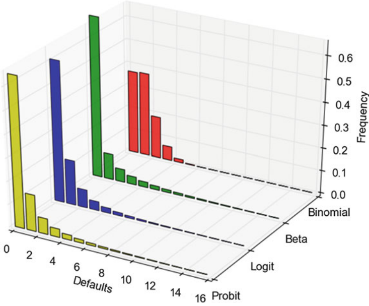
Fig. 3.5 Comparing default probability mass functions: This figure compares the four calibrated default probability mass functions: independent-default, beta-binomial, logit-normal, and probit-normal. All follow from the basic structure of equation 3.41.
