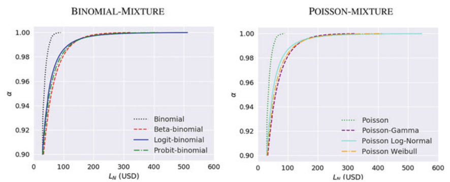
Fig. 3.7 Comparing tail probabilities: The underlying figures illustrate, for eight distinct binomial- and Poisson-mixture models, the structure of tail probabilities for our base portfolio example. As we incorporate default dependence and employ a common calibration, the general form is similar across all models. As we move further into the tail, however, significant differences arise.
