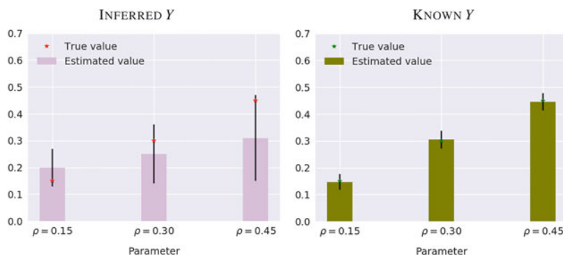
Fig. 10.14 Lost in translation : Although we do not observe the latent state variables, we can approximate the uncertainty with their inference. This is done by using the true, unobserved values; this is only possible, because we have simulated our underlying data.
