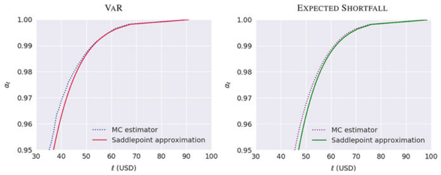
Fig. 7.8 Independent-default tail-probability and shortfall-integral approximations: This figure outlines—again for our usual 100-obligor example portfolio—the saddlepoint tail-probability and shortfall-integral approximations compared with a Monte Carlo simulation employing the usual 10 million iterations. Both approximations are extremely fast and quite accurate.
