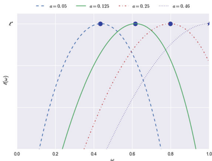
Fig. 10.7 Fixed a CreditRisk+ likelihood functions : This graphic illustrates four alternative, normalized, one-dimensional log-likelihood functions for distinct fixed choices of a . This permits us to assess their regularity and degree of informativeness.
