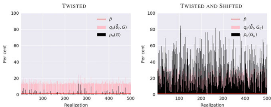
Fig. 8.12 Twisting and shifting : This figure illustrates the average unconditional, untransformed conditional, and transformed conditional default probabilities in the context of a one-factor Gaussian threshold model for two cases. The first involves solely an Esscher transform of the conditional default probabilities. The second is a simultaneous twist and shift of the same probabilities. Note the dramatically more extreme average conditional probability of default in the latter case.
