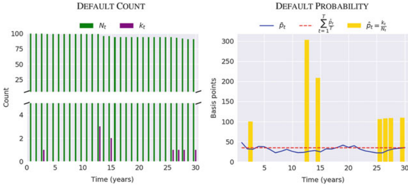
Fig. 10.3 Aggregate default data : These two figures summarize the intertemporal evolution of the number of credit counterparties, the number of defaults, the default rate, and the default probabilities. As default is a relatively rare event, its incidence is unsurprisingly infrequent.
