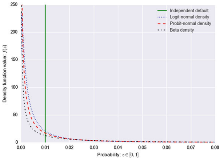
Fig. 3.4 Comparing default-probability densities: This figure compares the four calibrated default probability density function—including the trivial independent-default constant-parameter binomial model. Despite a common calibration, each choice has slightly different implications for default probabilities and hence one’s risk-measure estimates.
