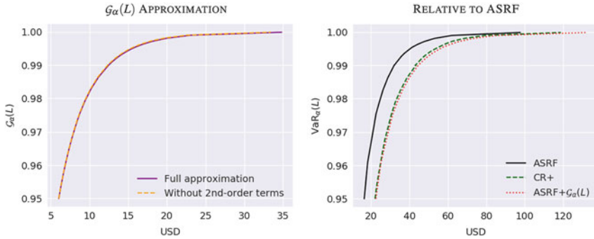
Fig. 6.12 G_\alpha(L) accuracy: The underlying figures focus on two questions. The first is: does the CreditRisk+ granularity adjustment provide a sensible approximation of concentration risk? Second, it asks: how important is the simplification in equation 6.72?
