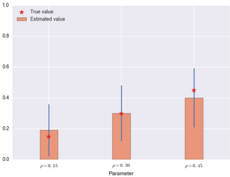
Fig. 10.5 Single-parameter estimates : Here we observe the true and estimated parameters for our single-parameter simulation study. The blue lines indicate, using observed noise in optimization results, an indication of the uncertainty in the maximum-likelihood estimates.
