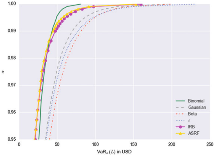
Fig. 6.5 Comparative tail probabilities: To put the Basel IRB estimates into context, this figure provides a comparative analysis of the tail probabilities associated with a broad range of relative model. In all cases, save the IRB and ASRF models, the expected loss has been subtracted to generate economic-capital estimates.
