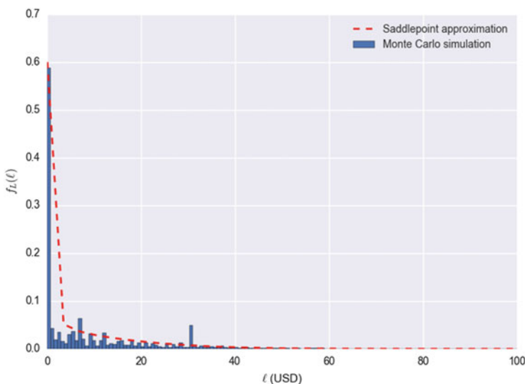
Fig. 7.7 Independent-default density approximation: This figure illustrates, for our running portfolio of 100 randomly generated heterogeneous exposures and default probabilities, density approximation. The density approximation, f_L(\ell) , is compared with a Monte Carlo binomial independent-default simulation employing 10 million iterations.
