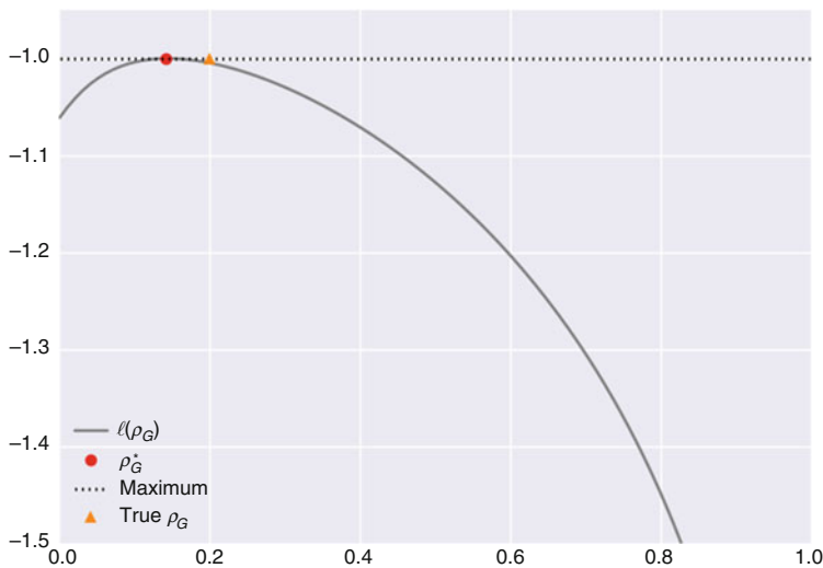
Fig. 10.4 Single-parameter likelihood function : Using the data from Fig. 10.3, this graphic traces—over the permissible domain of the parameter, \rho \in [0, 1] —the shape of the log-likelihood function. It also indicates the estimated and true population parameters. The log-likelihood appears to be regular.
