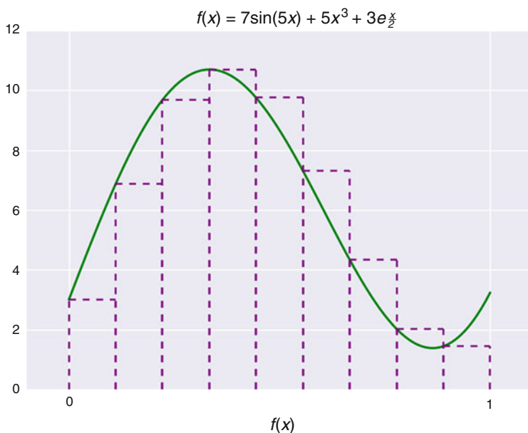
Fig. 8.2 A simple, but effective, approach: The underlying figure summarizes a naive, but effective, approach to numerical integration. The interval is partitioned into a number of non-overlapping sub-intervals; the area of each sub-interval is approximated by a rectangle.
