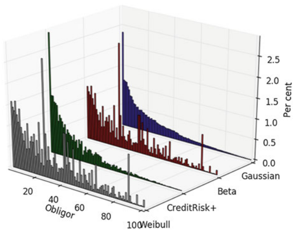
Fig. 7.15 Proportional saddlepoint shortfall contributions: This figure highlights ordered—following the Gaussian threshold model—expected-shortfall contributions for all models and all obligors. It is interesting to examine how the various models have different implications for the structure of credit-counterparty risk.
