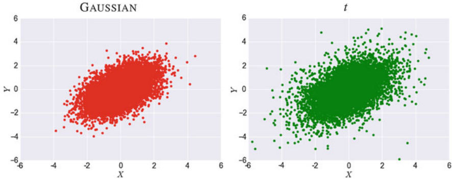
Fig. A.1 Bivariate scatterplots : The underlying figures use algorithm A.1 to illustrate the simulation of 10,000 bivariate Gaussian and t random-variate outcomes. The correlation coefficient, \rho , is set to 0.5 and the degrees of freedom parameter, \nu = 9 .
