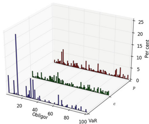
Fig. 7.10 VaR contribution perspective : This figure compares, in percentage terms, the unconditional default probabilities, obligor exposures, and VaR contributions for the 99.99th percentile in the independent-default binomial model. The combination of these three factors provided significant insight into the model output.
