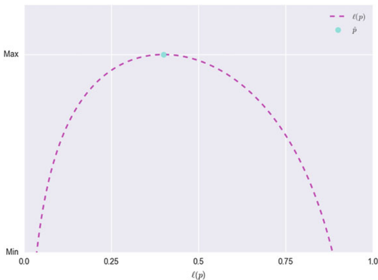
Fig. 9.10 Binomial likelihood : This figure plots the binomial log-likelihood function—conditional on the data in equation 9.65—across the range of possible population parameter values. While the likelihood clearly has a quadratic form, which implies regularity, it is relatively flat around its maximum. This is due to the small sample size.
