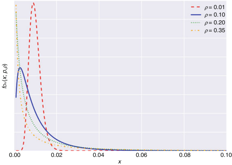
Fig. 4.4 Different limit-loss densities: This figure graphs the limit-loss density derived in equation 4.55 for different settings of the parameter, \rho . In all cases, p = 0.01 .
