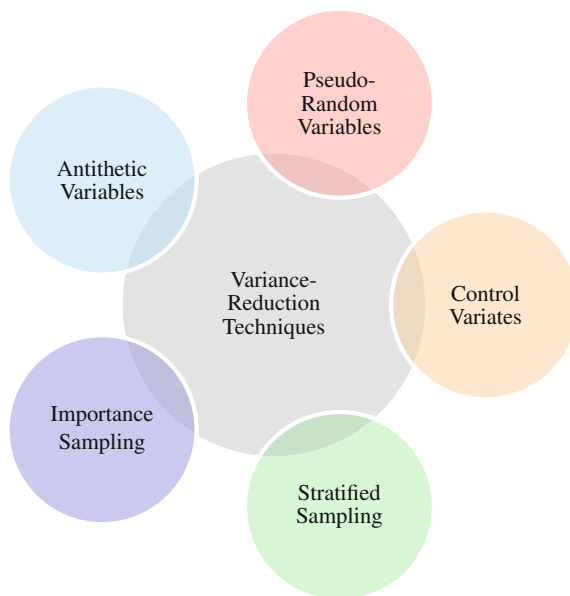
Fig. 8.8 Variance-reduction techniques : This figure illustrates schematically a range of alternative variance-reduction techniques. Not all methods perform equally well for every problem. The greatest improvements generally arise from exploiting knowledge of one's specific problem.
