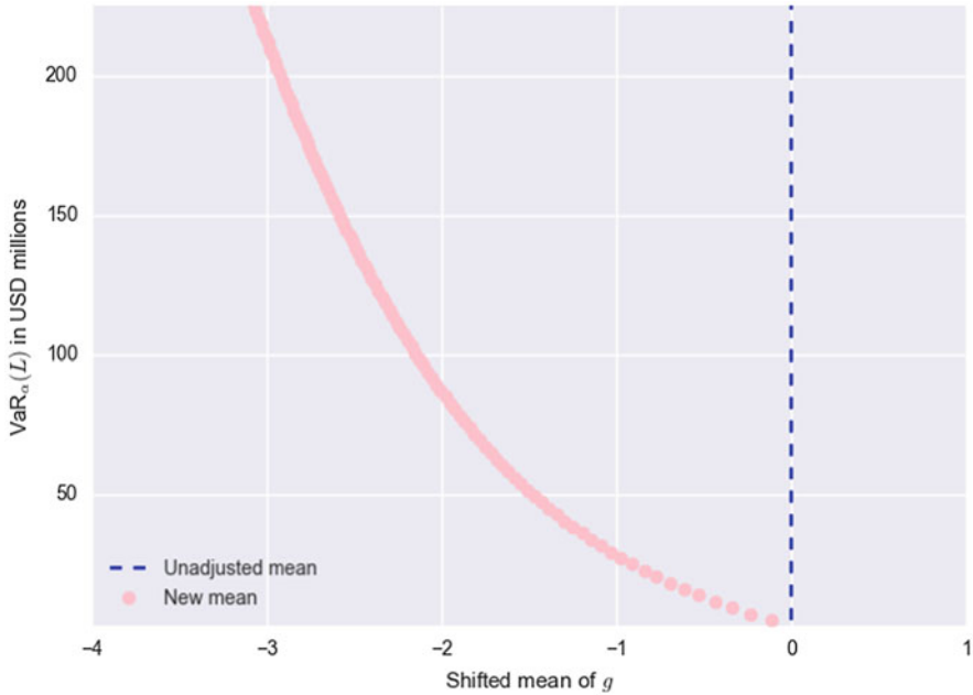
Fig. 8.13 The shifted mean: This figure illustrates, in the context of the one-factor Gaussian threshold model, the relationship between the choice of \ell and the shifted mean, \mu .
